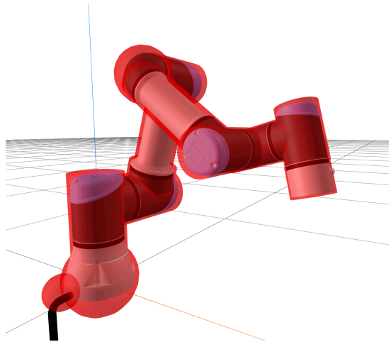
Figure 5.4 - Visualizing the visual and collision geometries for the UR3e.
